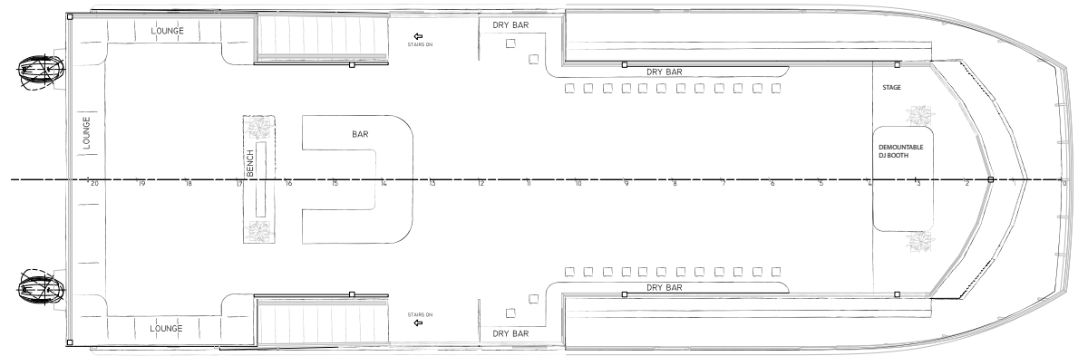
3 UPPER DECK
