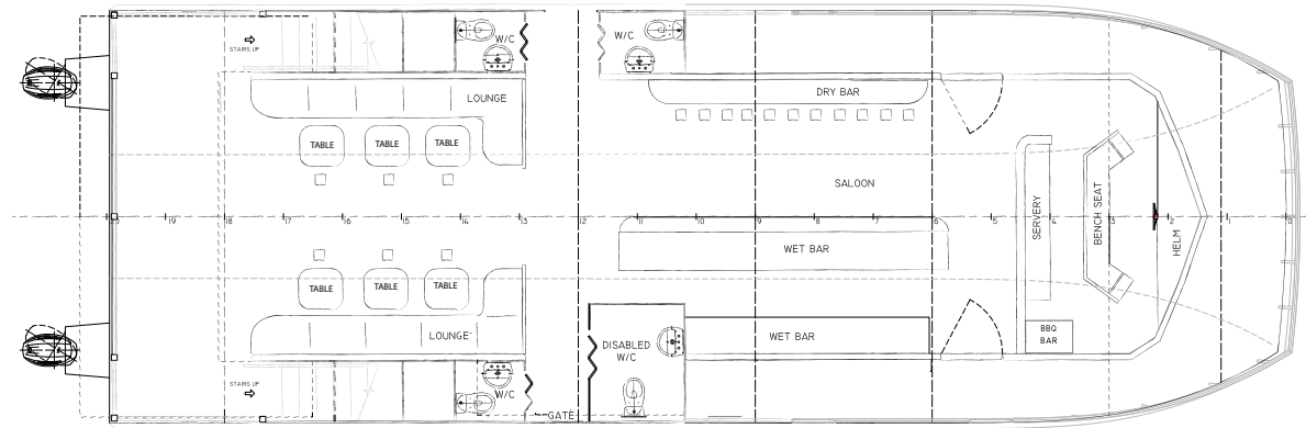
2 MAIN DECK
